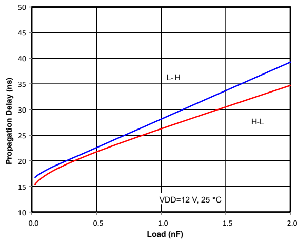
Figure 3.9. Propagation Delay vs. Load
