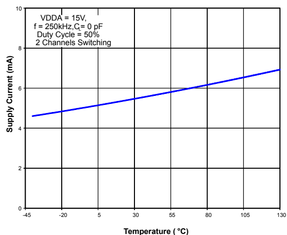
Figure 3.23. Supply Current vs. Temperature
